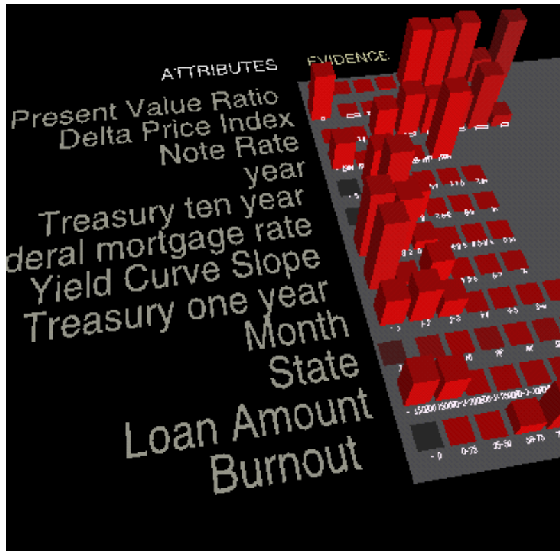
Figure 5: The simple/naive-Bayes model for prepayments.
